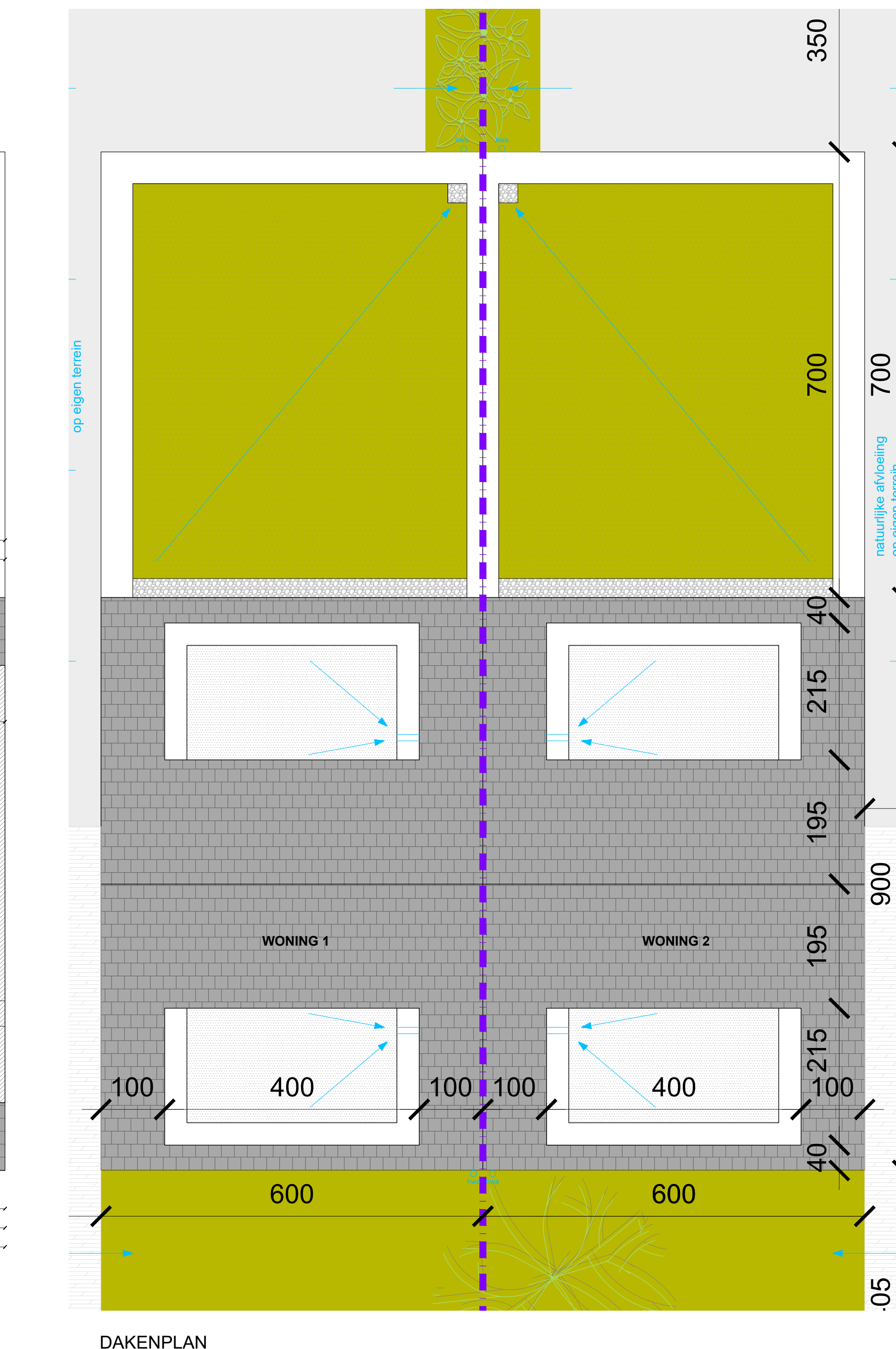
DAKENPLAN
