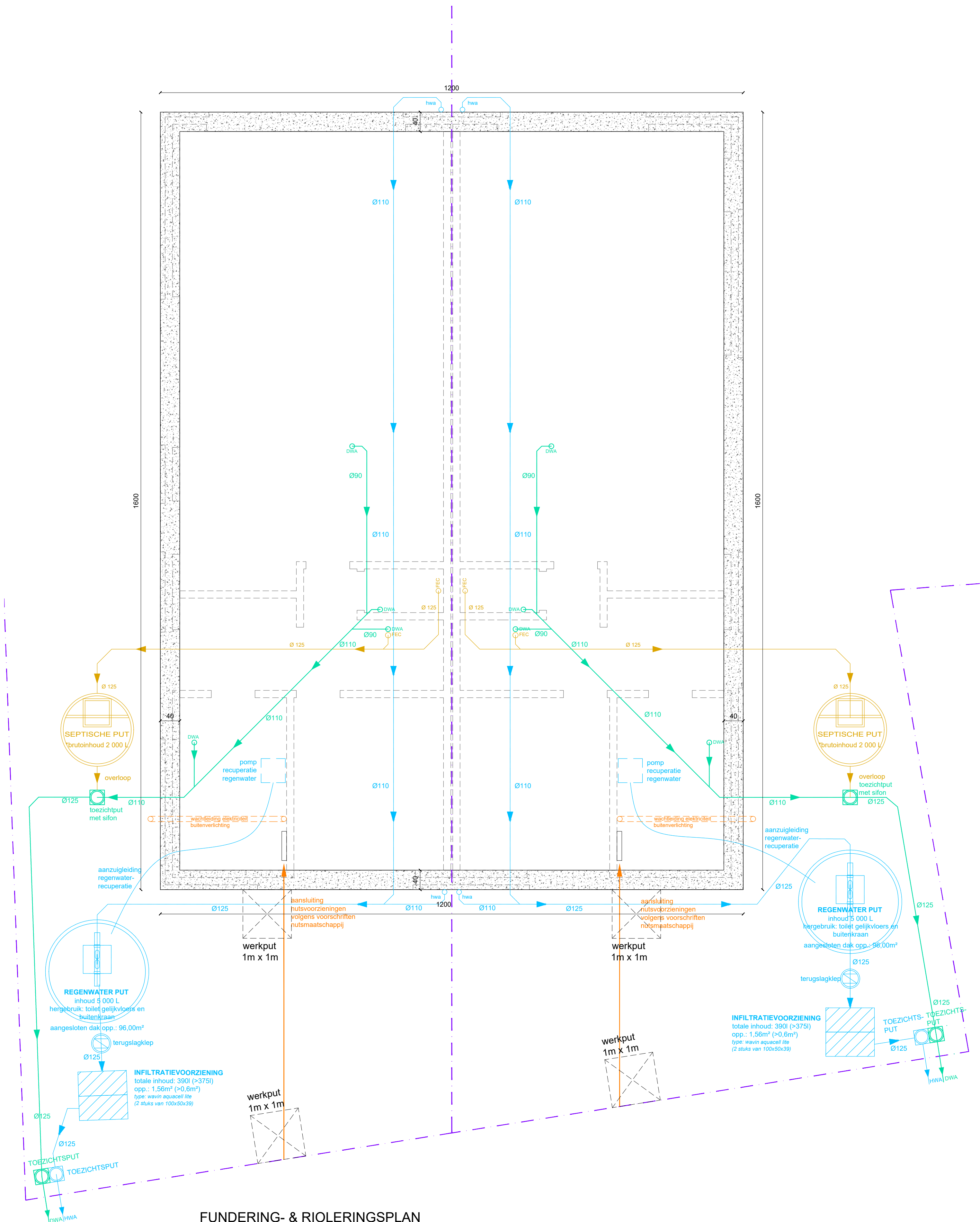
FUNDERING- & RIOLERINGSPAN
